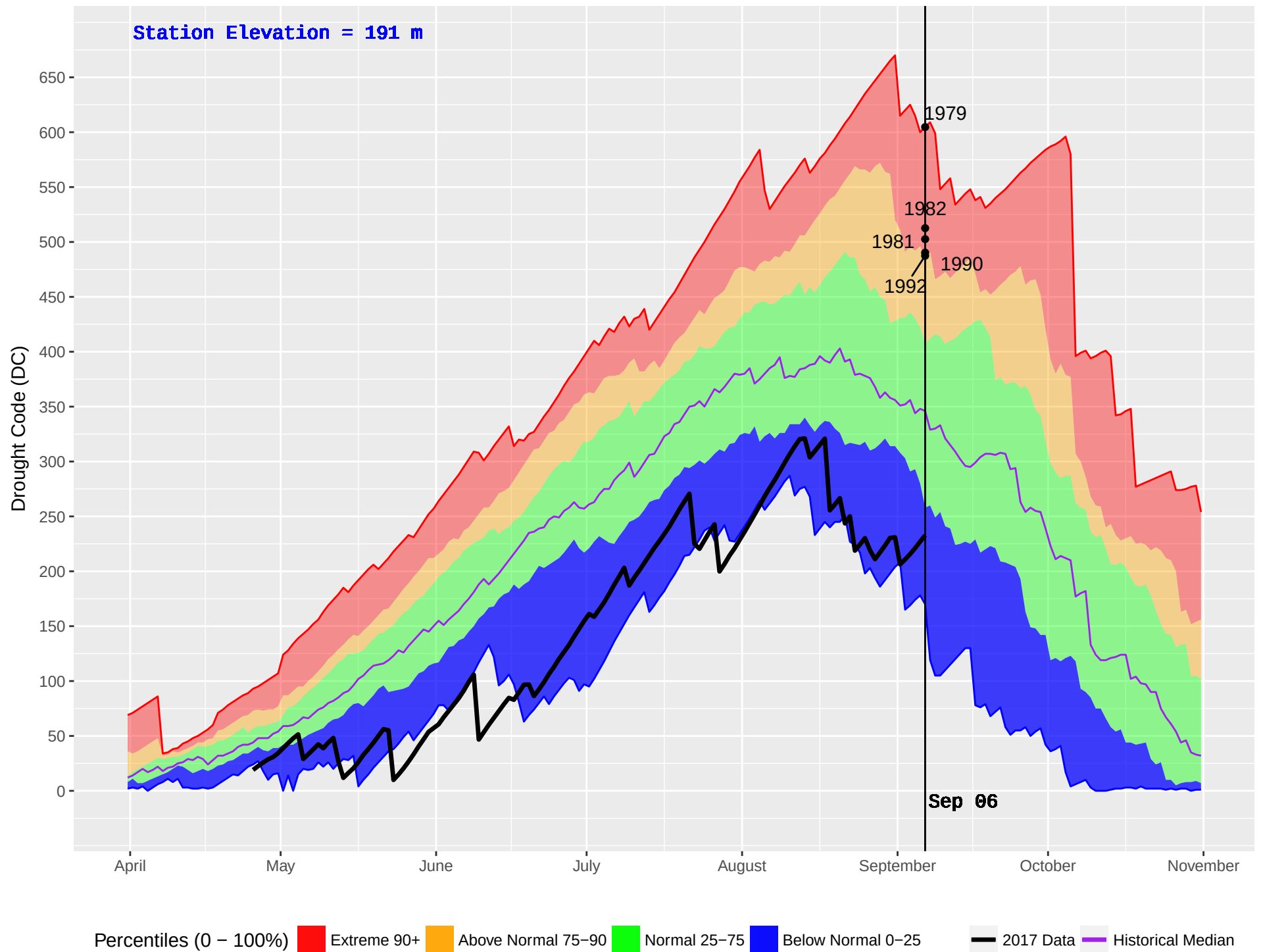
NASS CAMP (427) : Historical (1970–2016) and Current (2017) Noon Drought Code (DC)
