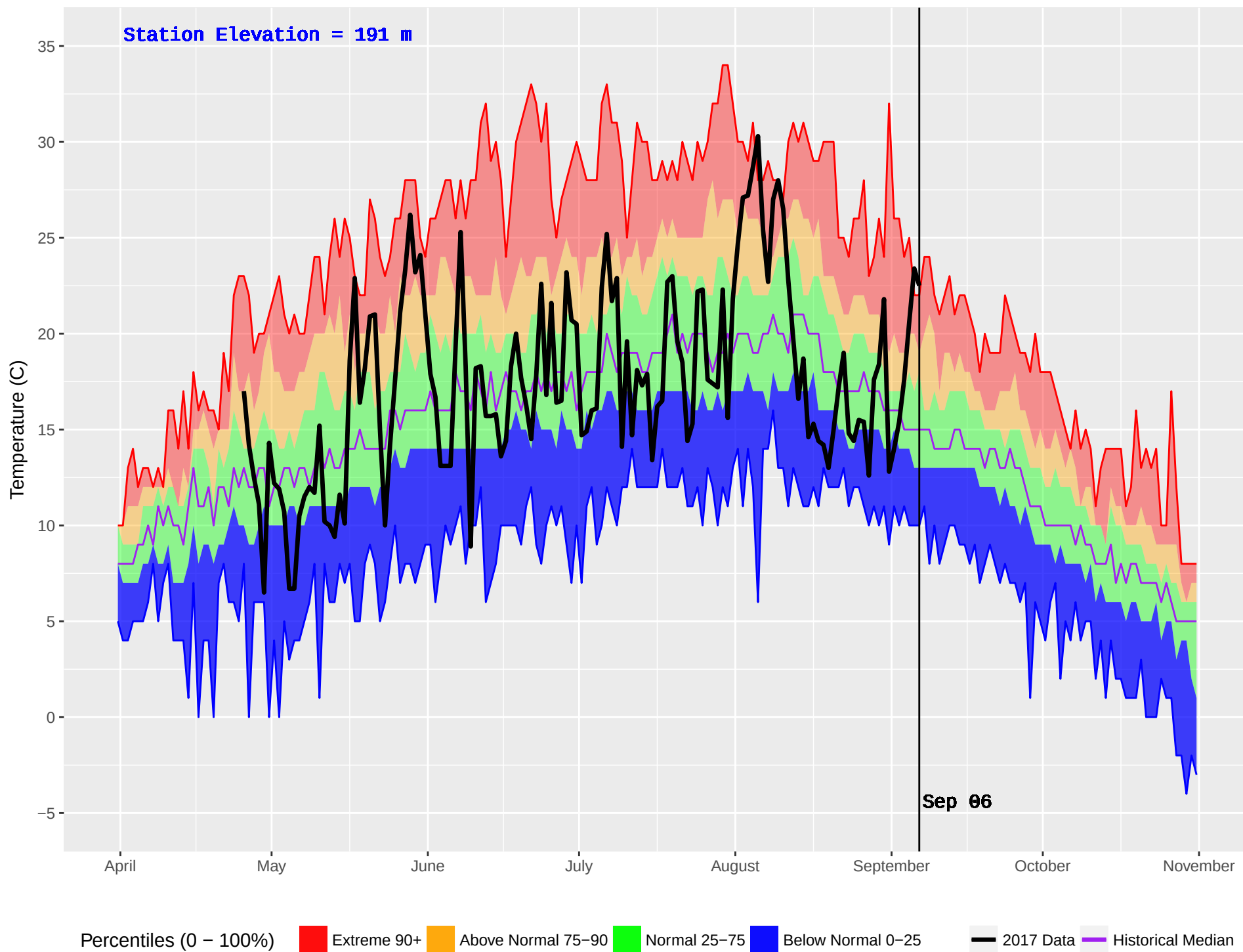
NASS CAMP (427) : Historical (1970–2016) and Current (2017) Noon Temperature
